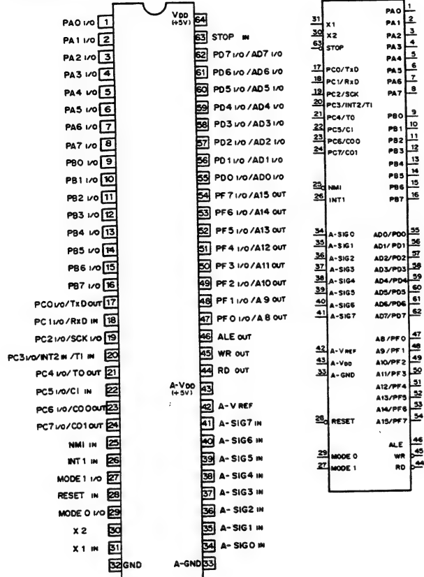
uPD78C10G C-MOS SINGLE CHIP 8-BIT MICROPROCESSOR WITH A/D CONVERTER — TOP VIEW —
